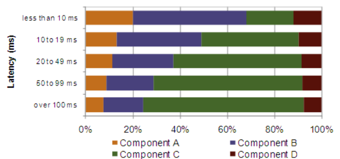
Fig. 1 – Sumerian visualisation for end-to-end latency distribution across components
