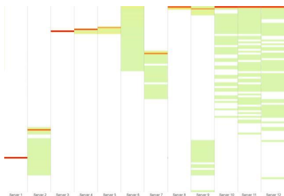
Fig. 2 – Sumerian distribution intensity map showing CPU utilisation
